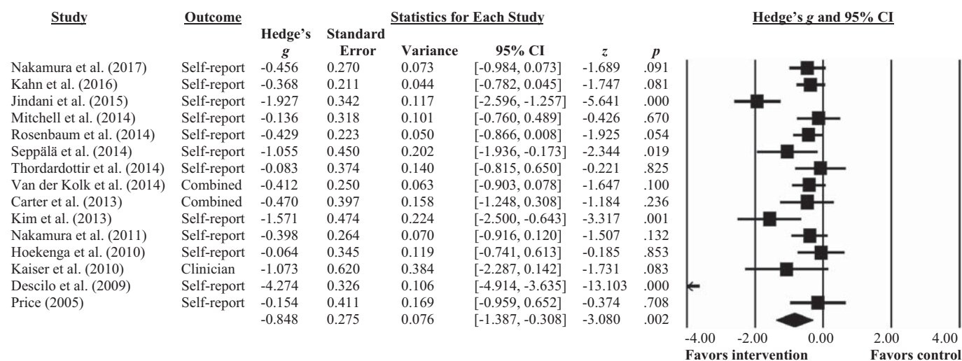
Figure 2. Meta-analysis of all included studies.
